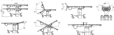
HFMH600 Manual Hydraulic Operating Table
